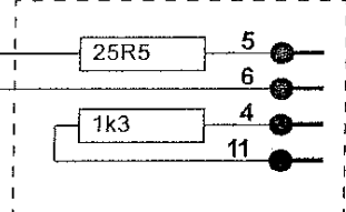
Oxford Connector
