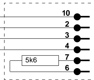
Oxford Connector
