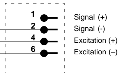
Corometrics Connector
