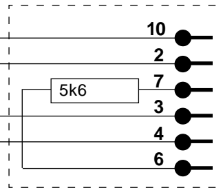
Oxford Connector
