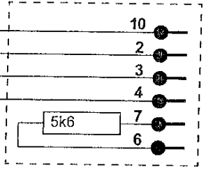
Oxford Connector
