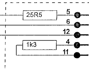
Oxford Connector
