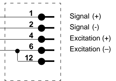
Corometrics Connector
