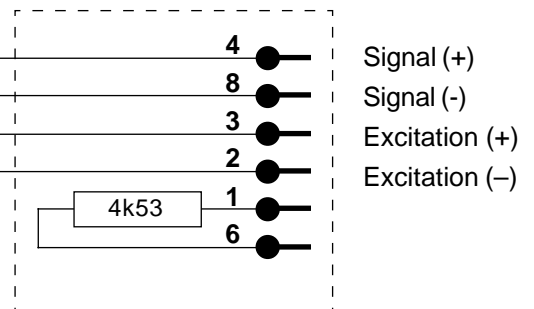
Agilent Connector
