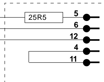
Oxford Connector
