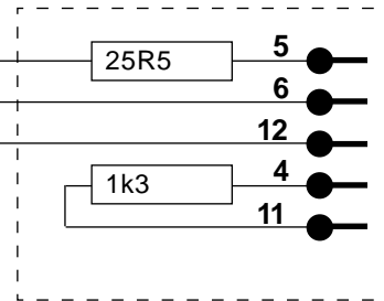
Oxford Connector
