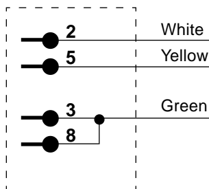
mini-DIN Connector
