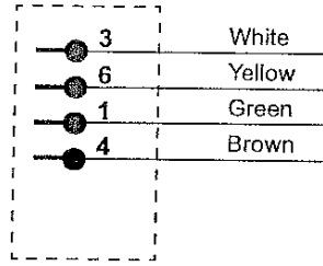
mini-DIN Connector
