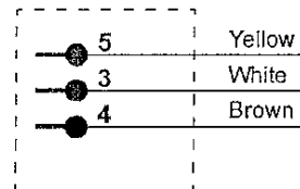
mini-DIN Connector
