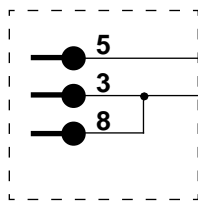
mini-DIN Connector
