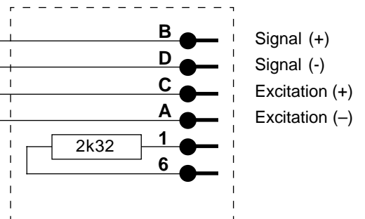
Agilent Connector
