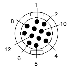
Solder side
