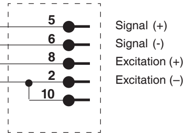
Corometrics Connector
