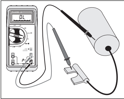
Figure 10: Checking condenser leakage Check for leaking condensers with the Ohms function. As the condenser charges up, the resistance should increase to infinity. Any other reading indicates that you should replace the condenser.
