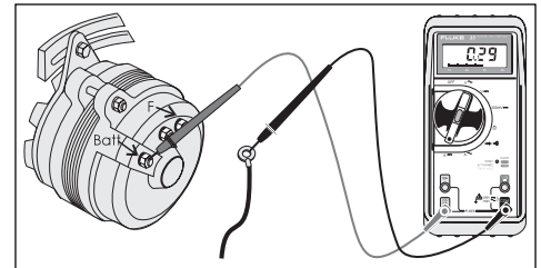
Figure 6: Alternator leakage current To check alternator diode leakage, connect the multimeter in series with the alternator output terminal when the engine is not running. Leakage current should be a couple of milliamps at most; more often, it will be on the order of 0.5 milliamps. Use care when disconnecting the alternator output wire; make sure the battery is disconnected first. A leaking diode can discharge the battery when the engine is off.
