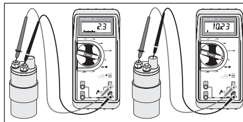
Figure 9: Measuring internal coil resistance If you suspect a malfunctioning ignition coil, check the resistance of primary and secondary windings. Do this when the coil is hot, and again when it is cold. Also measure from the case to each connector. The primary windings should have a very low resistance, typically from a few tenths of an ohm to a few ohms. The secondary windings have a higher resistance, typically in the 10 kΩ to 13 kΩ range. To get the actual figures for a specific coil, check the manufacturer's specs. But as a rule of thumb, primary windings range from a few tenths of an ohm to a few ohms, and secondary winding may be 10 kΩ or more.
