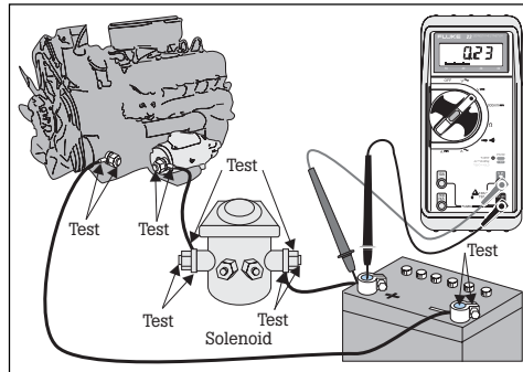
Figure 8: Testing for excessive voltage drop Determine if there is resistance in the circuit by measuring the voltage drop across each connection and component in the starter circuit while cranking the engine. Measure the voltage drop between the battery post and the connecting cable, the solenoid posts and the wires that attach to them, and across the solenoid itself. Also check the connection on the starter, alternator (feed and ground side) and the ground strap connection to the engine block. A logical test sequence would be to start by first measuring the battery voltage between + and - terminals when the starter is cranking. Then measure the voltage between the starter terminal and engine block when cranking. If the starter voltage is significantly less, use the above procedure to isolate the voltage drop.
