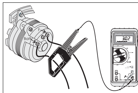
Figure 3: Verifying a good alternator The battery must be fully charged (see Figure 1). Run the engine and verify that no-load voltage is 13.8 to 15.3V (check as in Figure 1). Next load the alternator by turning on dc loads such as lights, radio, etc. Run the engine at 2000 RPM. Check the current with an i410 or i1010 current clamp.
