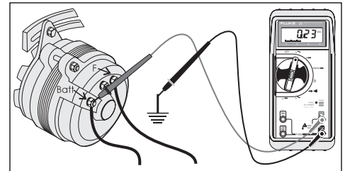
Figure 5: Checking ripple voltage Ripple voltage (AC voltage) can be measured by switching your DMM to AC and connecting the black lead to a good ground and the red lead to the "BAT" terminal on the back of the alternator, (not at the battery). A good alternator should measure less than 0.5 VAC with the engine running. A higher reading indicates damaged alternator diodes.
