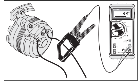
Figure 4: Checking field current Worn brushes limit field current, causing low alternator output. To test: load unit as in Figure 3 and measure field current with current clamp or use 10A jack on DMM. Readings range from 3 to 7 amps. On integral GM units: with alternator not turning, jump terminals #1 & #2 together and connect both to Batt + with DMM in series set to measure 10 amps. Field current should be between 2 & 5 amps, higher current with lower battery voltage. Control battery voltage by turning on lights, radio, etc.
