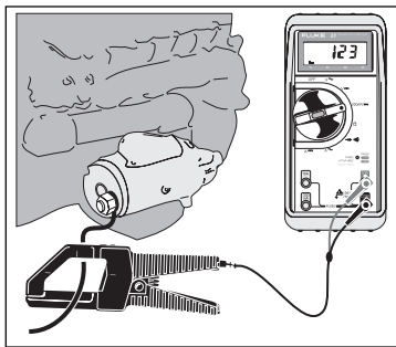
Figure 7: Measuring starter current draw Determine how much current the starter is drawing by using Fluke's i1010 Inductive Current Clamp on the starter cable. This accessory will allow the multimeter to measure starter current up to 1000 amps. Check manufacturer's specs for exact figures.
